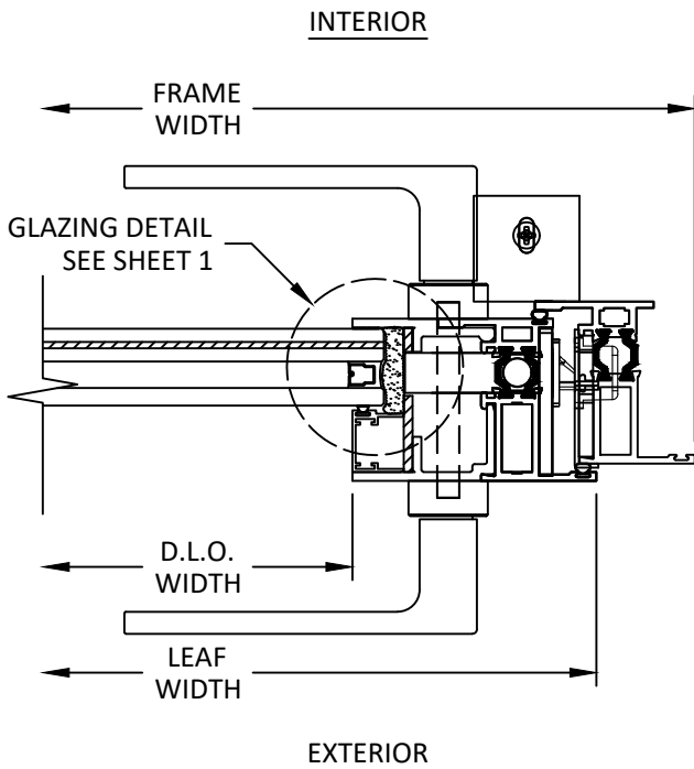
H 6 HORIZONTAL SECTION LOCK JAMB - LOCK
