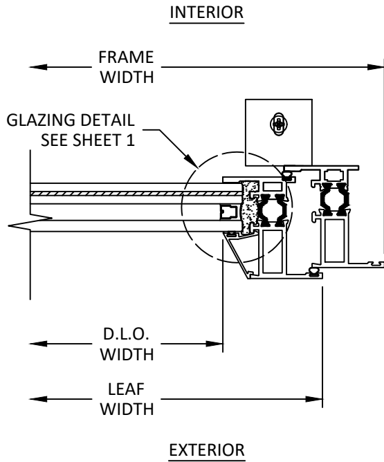
F 6 HORIZONTAL SECTION LOCK JAMB
